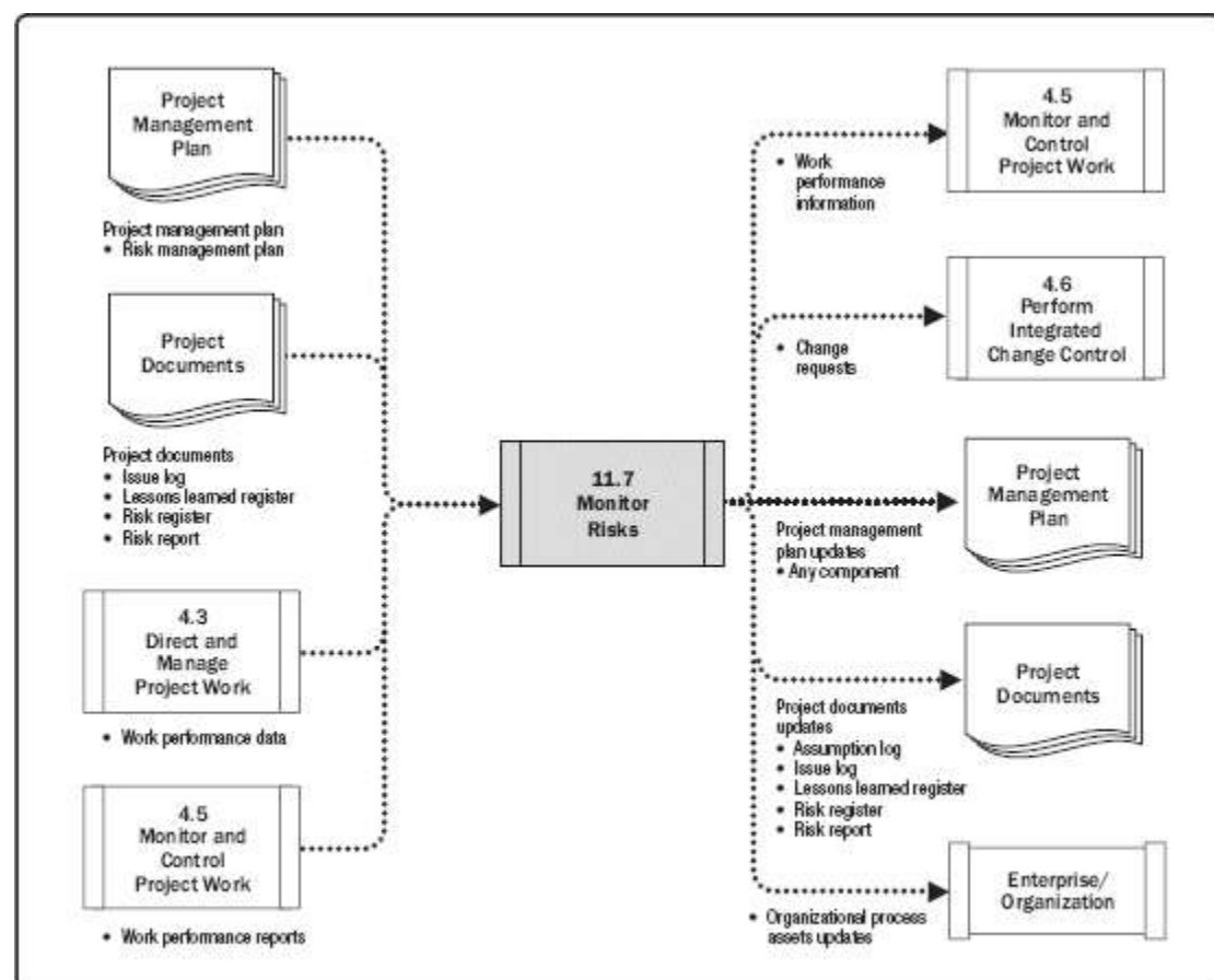
Figure 11-20. Monitor Risks: Inputs, Tools & Techniques, and Outputs
